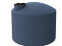
BT3000-S 3,000L/660Gal (Squat) Height 1,500mm Diameter 1,800mm Outlet 25mm Overflow 90mm
